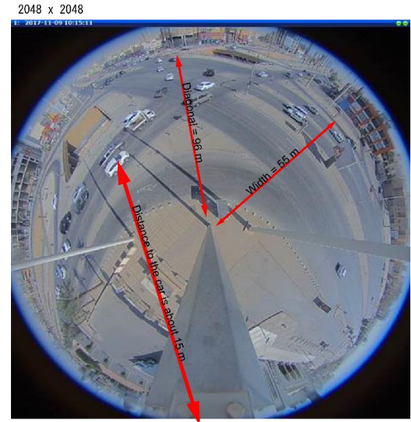
The camera is installed on a pole of 12 m high facing downward.
